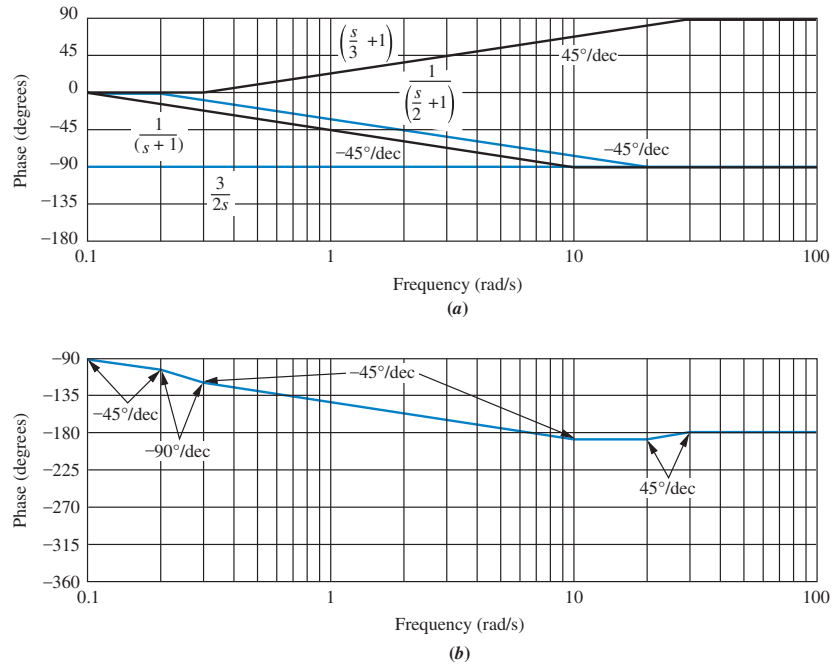
FIGURE 10.12 Bode phase plot for Example 10.2: a. components; b. composite
